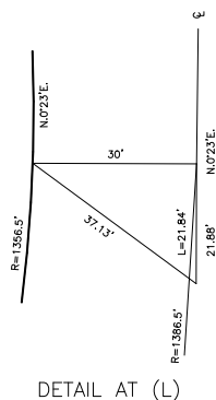
DETAIL AT (L)
